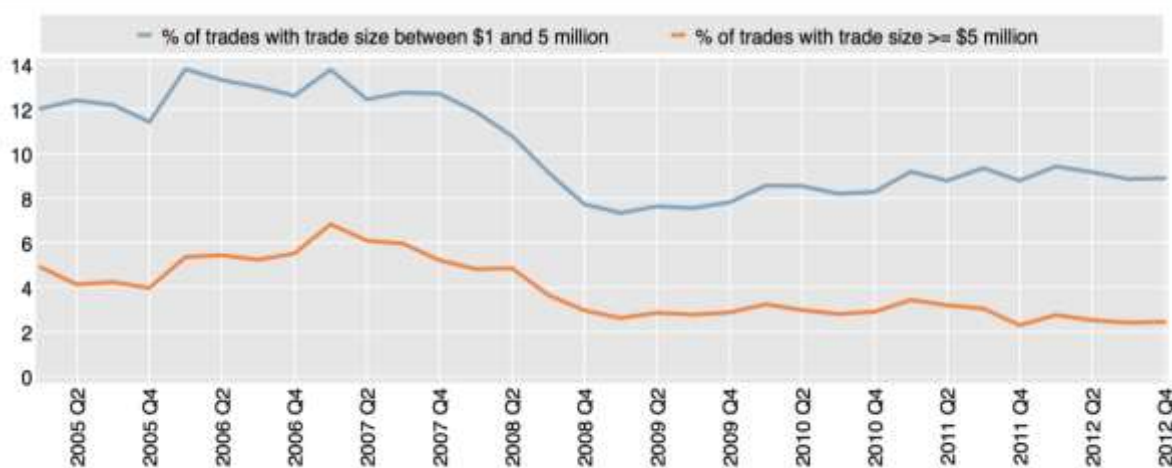
Figure 20. Percentage of large trades in the US
